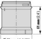
1160DIM-86 Line drawing
