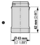
1160DIM-61 Line drawing
