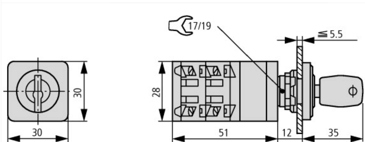
Key operation lock mechanism
