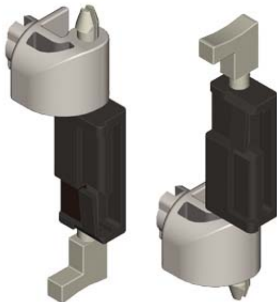
ALPHA, ACCESSORY SPARE HINGE FOR WALL/FLOOR- MOUNTED DB
