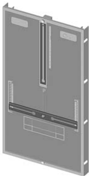
ALPHA 400 METER SUPPORT PLATE H=450MM, W=250MM DESIGN F. NORWAY
