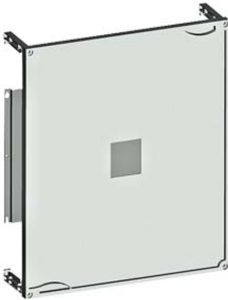
ALPHA 400/630 DIN, KIT FOR POWER CIRCUIT-BREAKER 3/4 POLE, 3VL400/630, H=600 W=250
