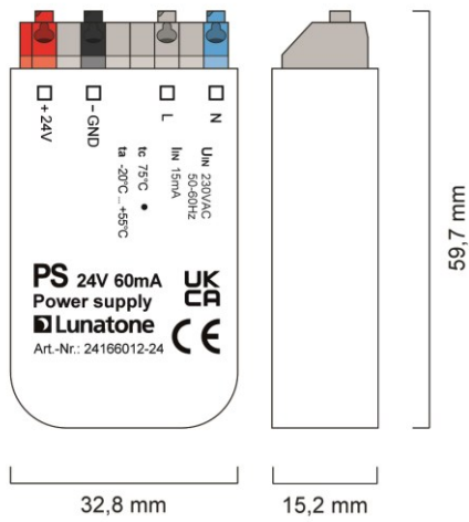
geometry PS24 60mA back box (24166012-24)
