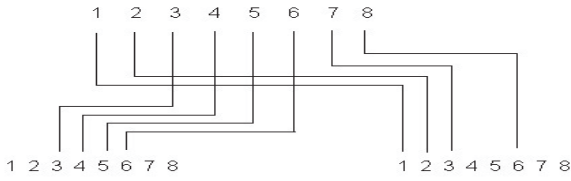
SPLITTLEDD TELE/DATA EL.NR 6970079
