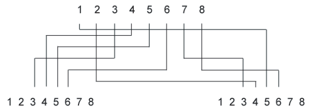
SPLITTLEDD 2xISDN EL.NR.6973658
