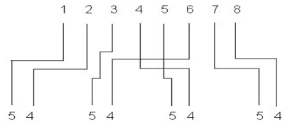
SPLITTLEDD 4XTELE EL.NR 697857
