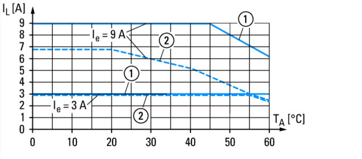
Electricity derating devices with EMS2-XTH adapter ① For devices installed with a minimum clearance of 20 mm ② For devices in direct sequence
