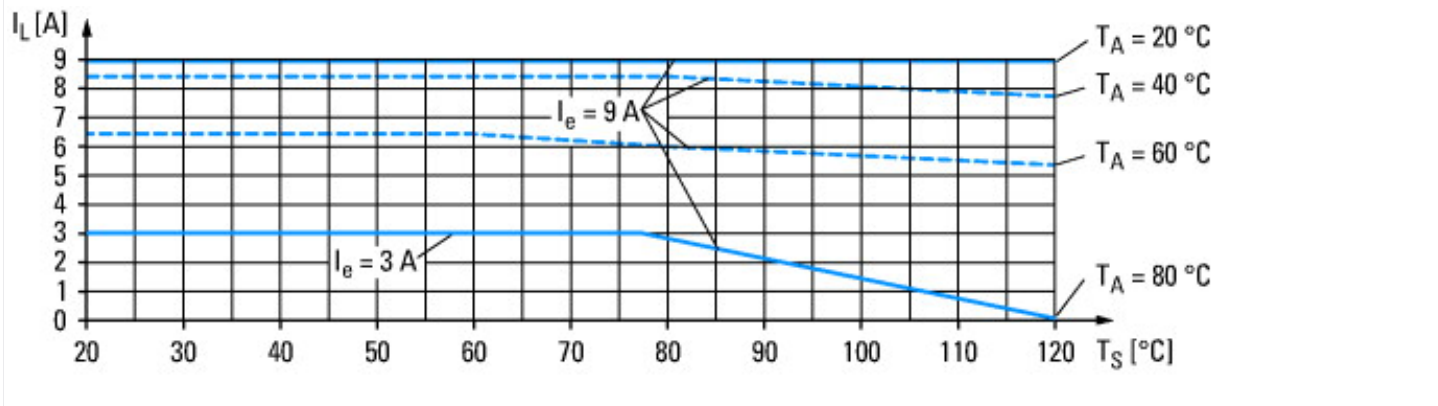
Electricity derating devices with EMS2-XBB or MSFS adapter Devices with I_e = 9 A that are installed with a minimum clearance of 20 mm. T_S = temperature of busbar T_A = ambient temperature in switch cabinet
