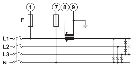
Fig. 6 AV5, AV6 balanced load
