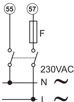
Fig. 21 D option. F = 250 V, 50 mA
