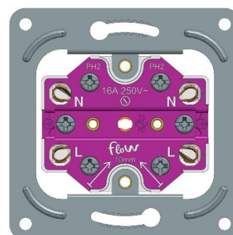
Base for double socket
