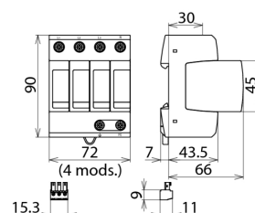
Dimension drawing DG M TNS 275 FM
