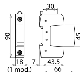
Dimension drawing DG S CI 275
