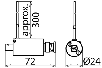
Dimension drawing UGKF BNC
