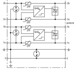
Basic circuit diagram DBX U4 KT DB S 0-180
