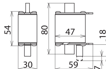
Dimension drawing VA NH00 280 FM
