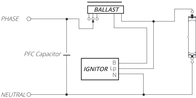
Typical impulser ignitor circuit
