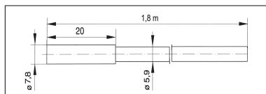
Dimensions of sensor
