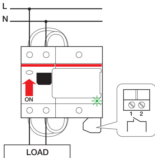
Wiring diagram for F2C-ARH and F2C-ARH-T
