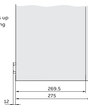
Side view With/without door
