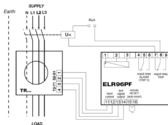
ELR96PF - undervoltage release wiring
