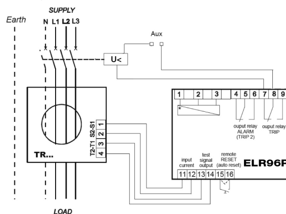
ELR96P - undervoltage release wiring
