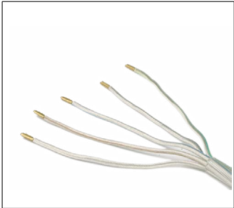
CABLE & WIRE 2,5 m cable 5 x 0.75 1.5 m wire Art.no. standard: E80000008 Art.no. w/ceiling cup: E80000009
