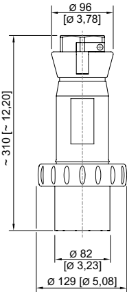
Dimensional Drawings (All Dimensions in mm [inches]) – Subject to Alterations
