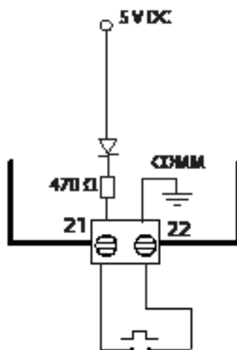
Figur 9: Digital Inngang, SE-C21-485-DS
