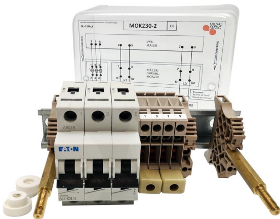
MOK 230V El.nr 82 001 00
