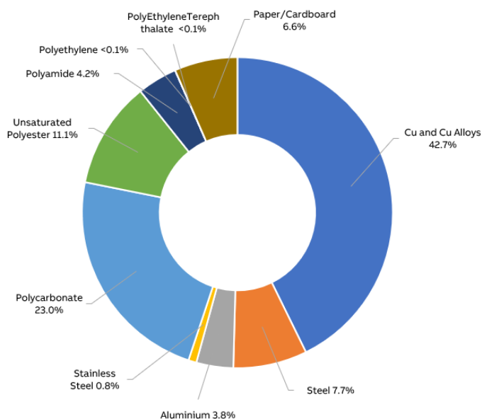
Figure 1: Composition of ZHBM1250A-3P-V Fuse Switch Disconnecter
