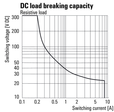
DC load limit curve Resistive load
