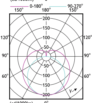
(cd/1000lm) 0° 0-180° 90-270°
