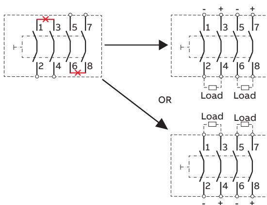
OTDCP_22_ ( U_e = 2 \times 1000\text{ V} )
