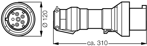
Plug 4/5-pole
