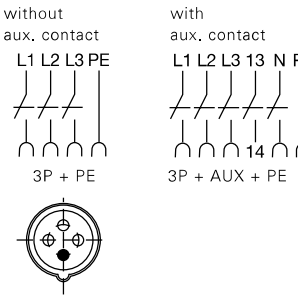
Plug 4/5-pole
