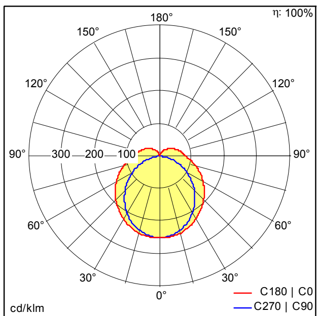
TE_ELSA_LED_600_1200_830_WH.Idt
