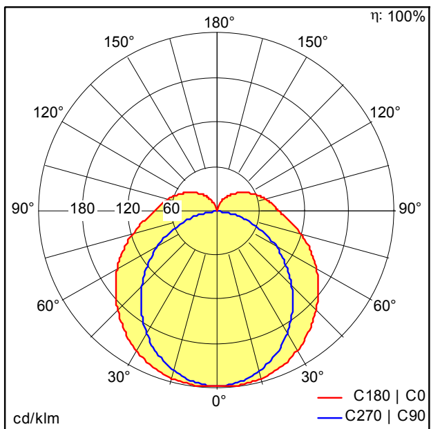
TE_ELSA_LED_450_800_830_MWS_WH.Idt
