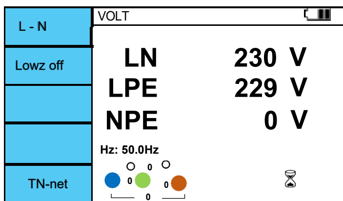
Figure 6.4.2 Voltage measurement screen.
