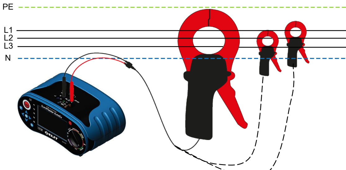
Figure 6.10.2 Adaptor/ Current Clamp connection.
