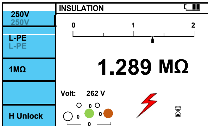
Figure 6.7.3 Insulation L-PE Measuring.
