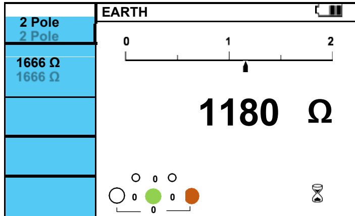
Figure 6.8.3 Earth Resistor 2Pole Measuring.
