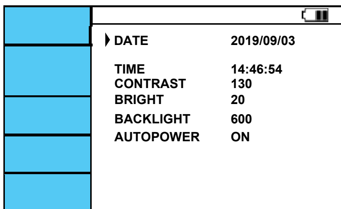
Figure 6.3.2 sysSet screen.
