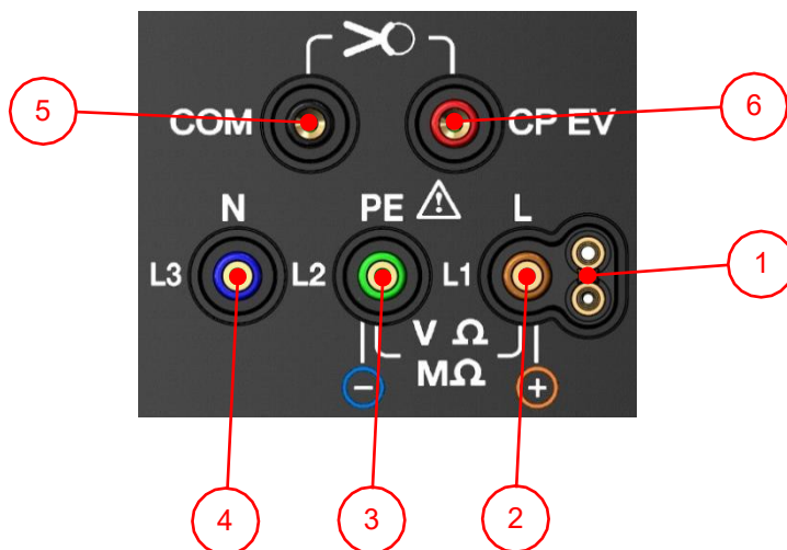
Figure 5.2 Input terminal.
