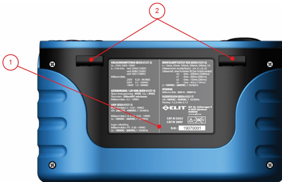
Figure 5.5 Bottom side.
