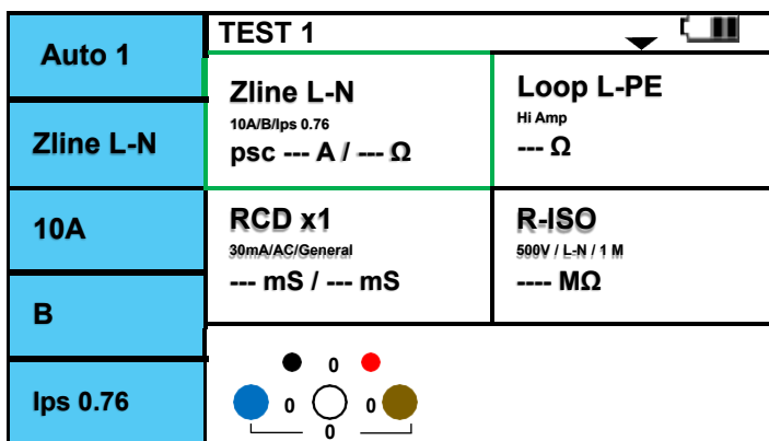
Figure 6.11.1 Auto test screen.
