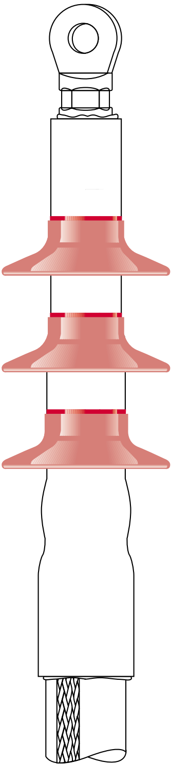
Polymeric or Paper Insulated Cable Outdoor Service
