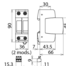
Dimension drawing DG M TT 2P CI 275 FM
