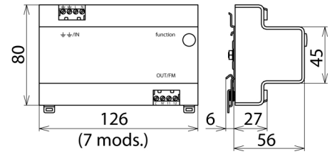
Dimension drawing SPS PRO
